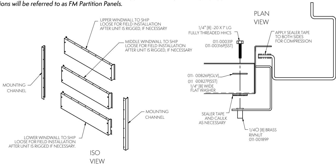
Figure 33 – Upper Partition/Firewall Installation in Field
