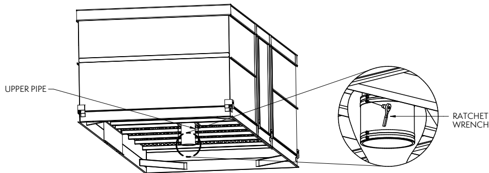
Figure 8 – Casing Bottom Inlet Piping
