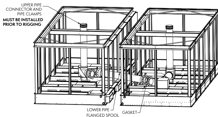
Figure 9 – Installation of Bottom Inlet Piping
