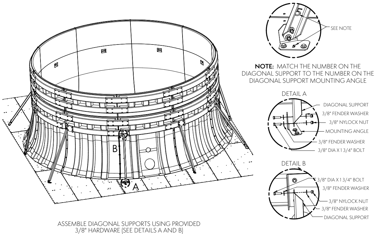
Figure 32 – Super Low Sound Fan Diagonal Supports
