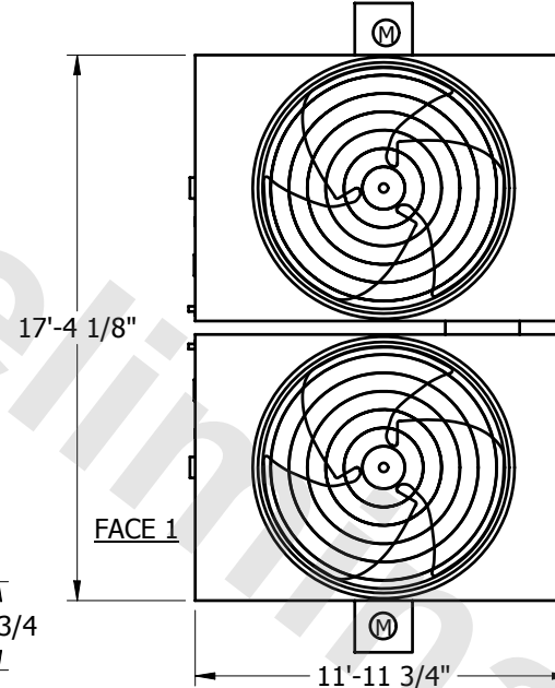
PLAN VIEW
